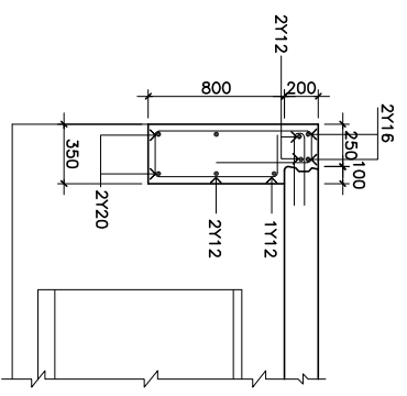
SECTION 5-5 CROSS SECTION THROUGH CAST IN SITU BEAM SCALE 1:25
