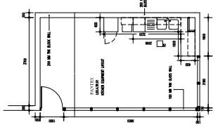
FIRST FLOOR PLAN SCALE = 1/8" = 1'-0"
