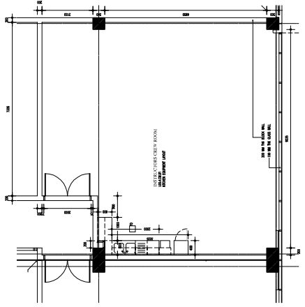
FIRST FLOOR PLAN SCALE = 1/8" = 1'-0"
