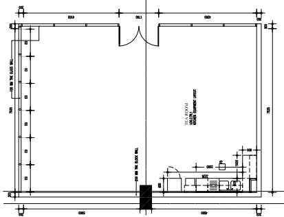
GROUND FLOOR PLAN SCALE = 1/8" = 1'-0"
