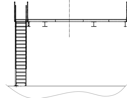
SECTION H-H.
