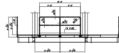
SECTION H-H.
