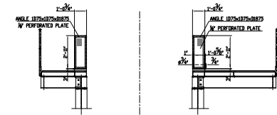
SECTION G-G.
