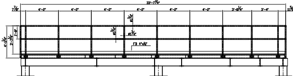
SECTION D-D.
