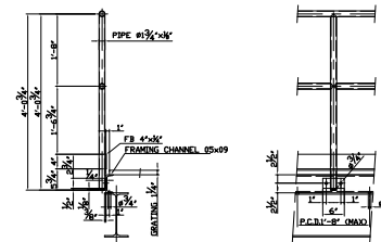
TYPICAL DETAIL SECTION
