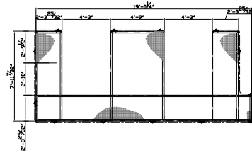
FRAMING CHANNEL 65x12
