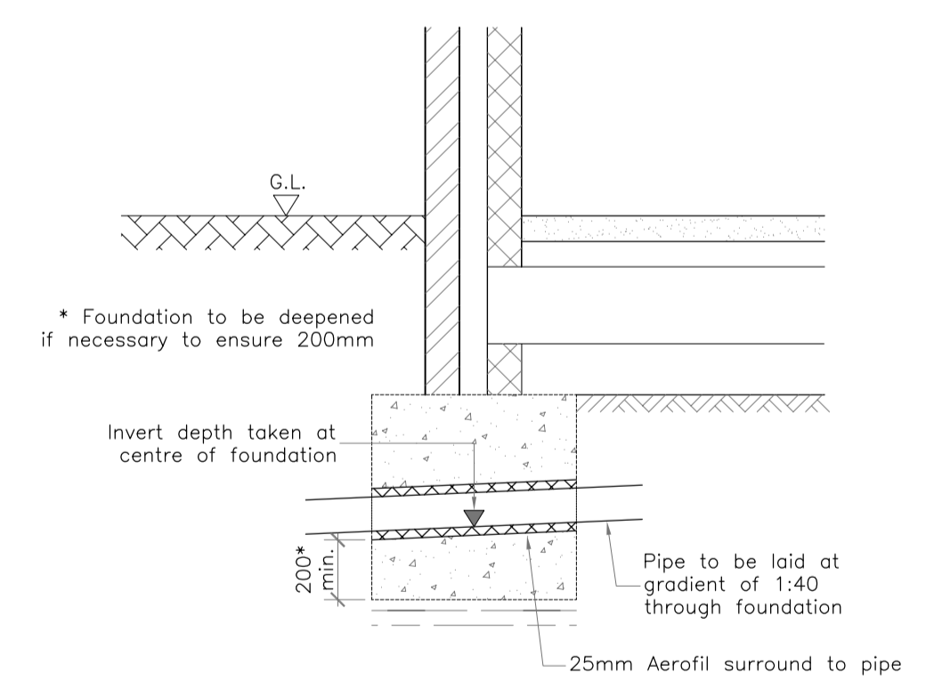
Typical Detail of Pipe Passing Through Foundation Scale 1:20
